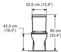
Vista Frontal / Front View
